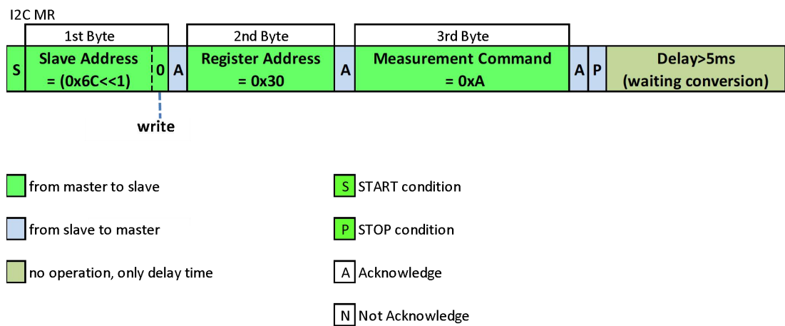
FIGURE 3: I 2 C MEASUREMENT REQUEST COMMAND
